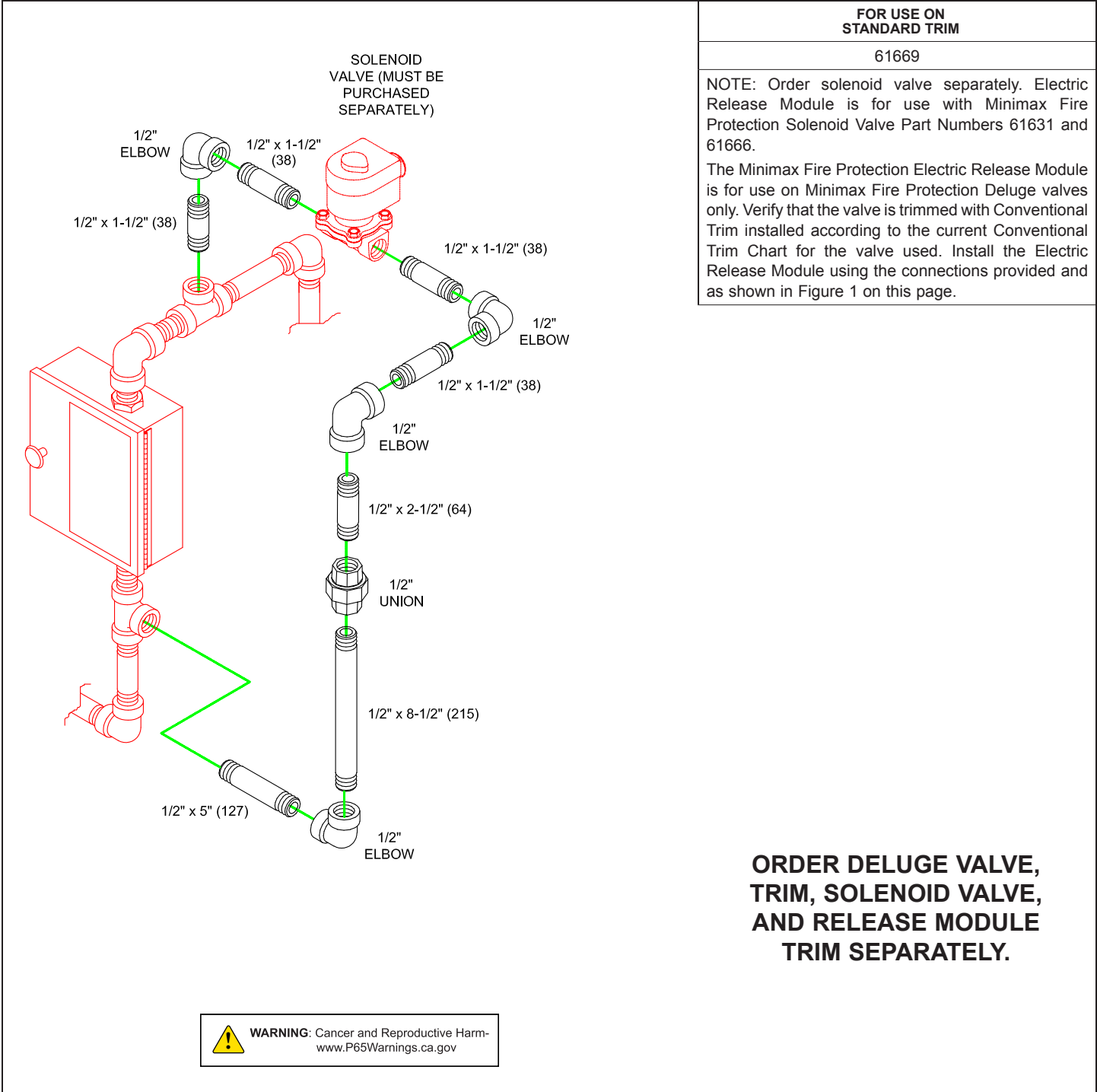
FIGURE 1: ELECTRIC RELEASE MODULE
